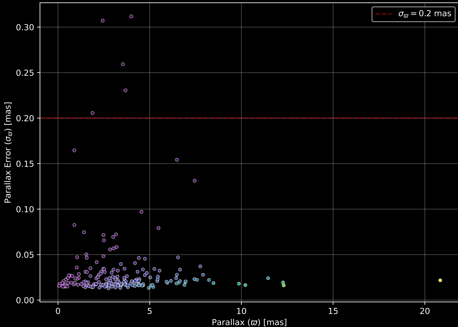
APOGEE DR17 Field: [168+63_MGA] Parallax Quality (n= 198)
