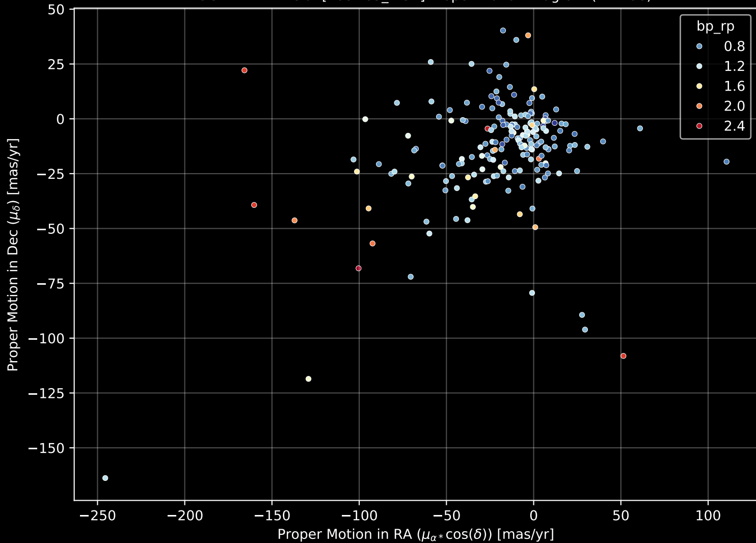
APOGEE DR17 Field: [168+63_MGA] Proper Motion Diagram (n= 198)
