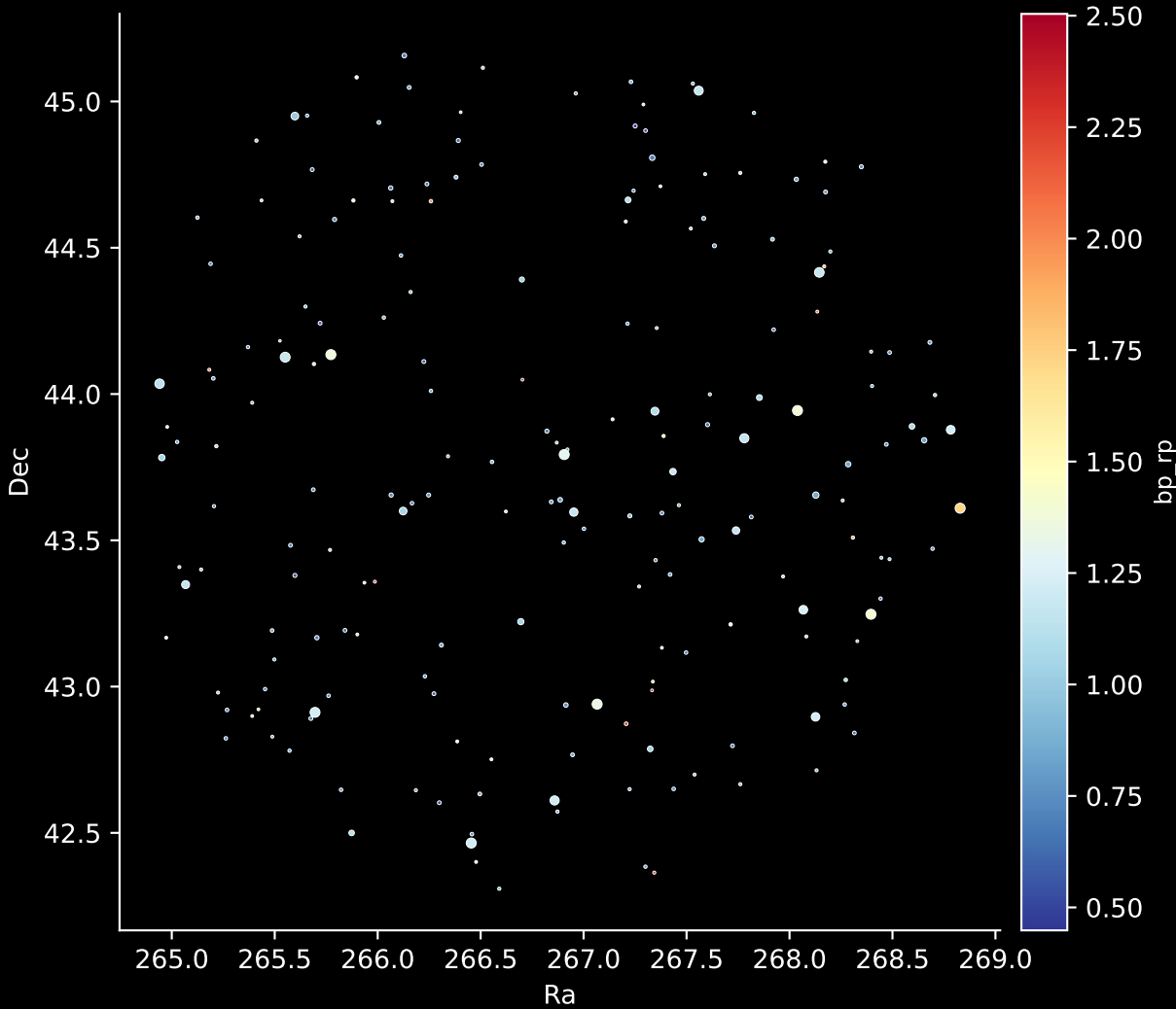
APOGEE DR17 Field: [168+63_MGA] Stars: 198
