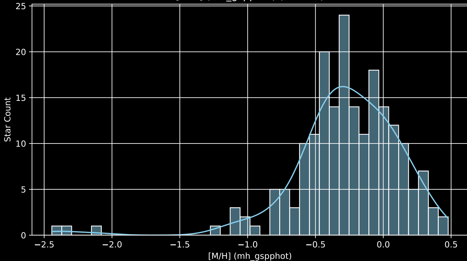
APOGEE DR17 Field: [168+63_MGA [M/H] (mh_gspphot) (n= 198)
