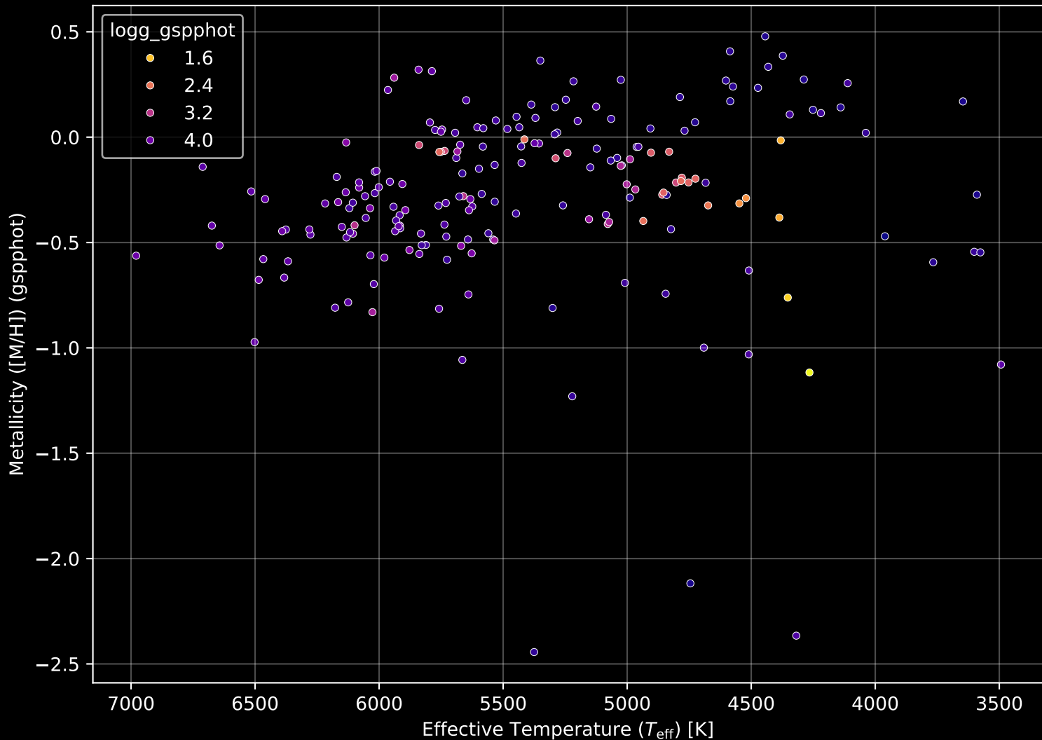
APOGEE DR17 Field: [168+63_MGA] Stellar Population Parameters (n= 198)
