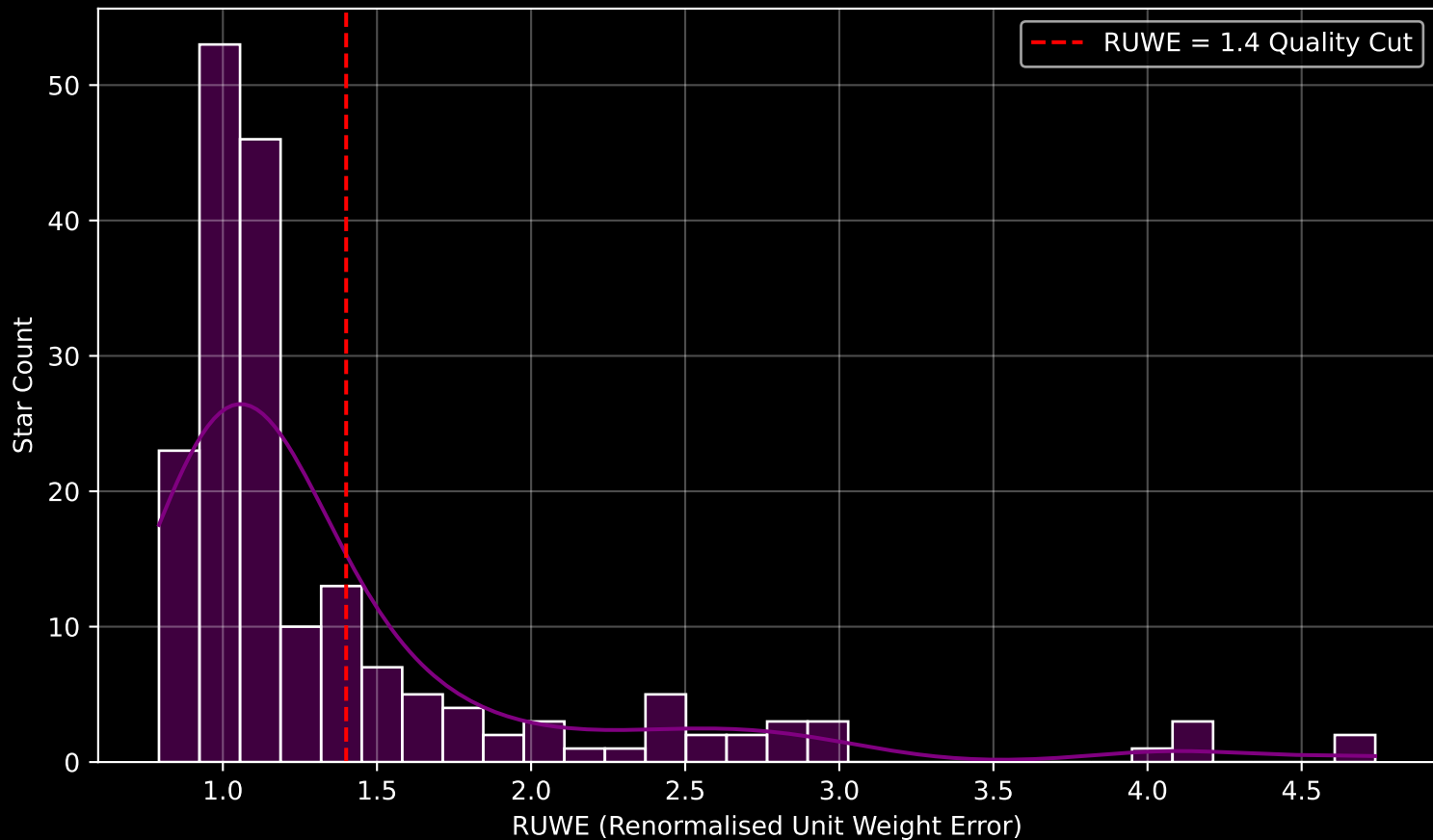
GAPOGEE DR17 Field [168+63_MGA] RUWE Distribution (n= 189)
