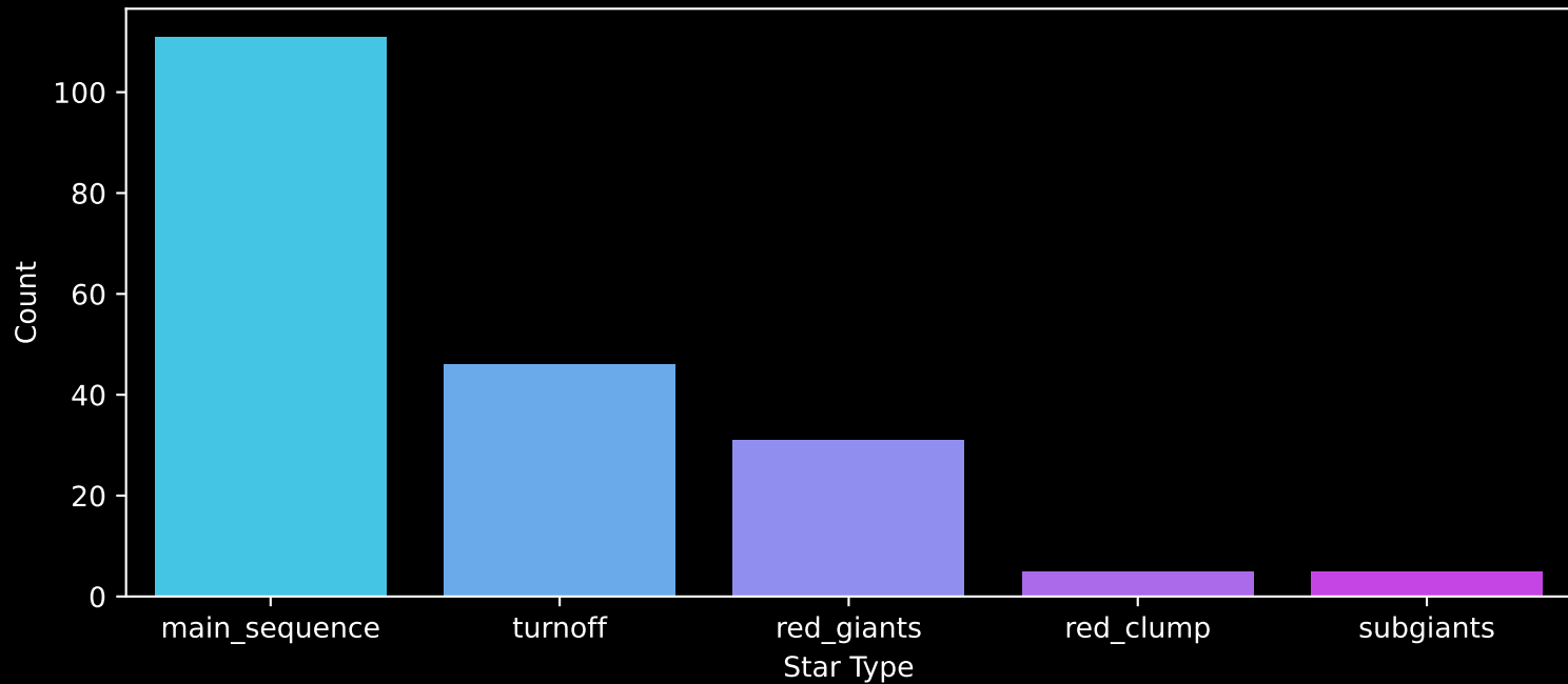
APOGEE DR17 Field: [168+63_MGA] Count plot of Star Type
